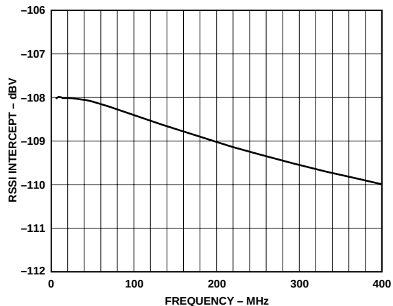
Figure 16. RSSI Intercept vs. Frequency Using Termination of 52.3 \Omega
