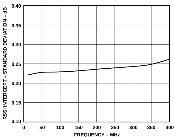
Figure 17. RSSI Intercept Standard Deviation vs. Frequency
