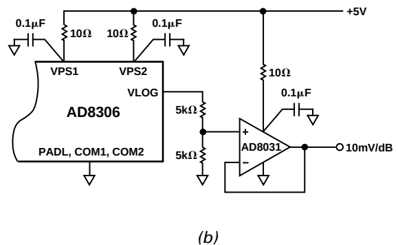
Figure 30. Altering the Logarithmic Slope
