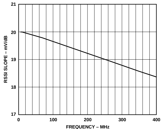
Figure 13. RSSI Slope vs. Frequency Using Termination of 52.3 \Omega
